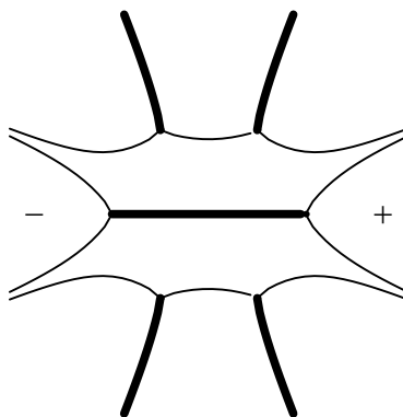
Fig. 8. d = 6, \ell = 3 .
