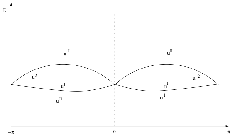
Fig. 2. Sections in the Brillouin zone.
