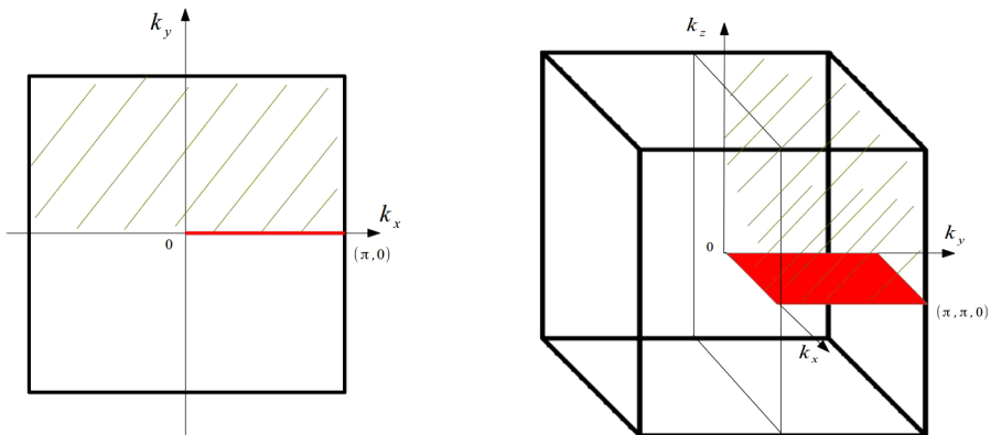
Fig. 1. (Color online) Effective Brillouin zone in 2d and 3d.
