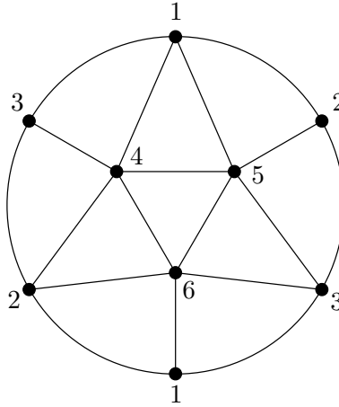
FIGURE 1. A triangulation of the real projective plane
