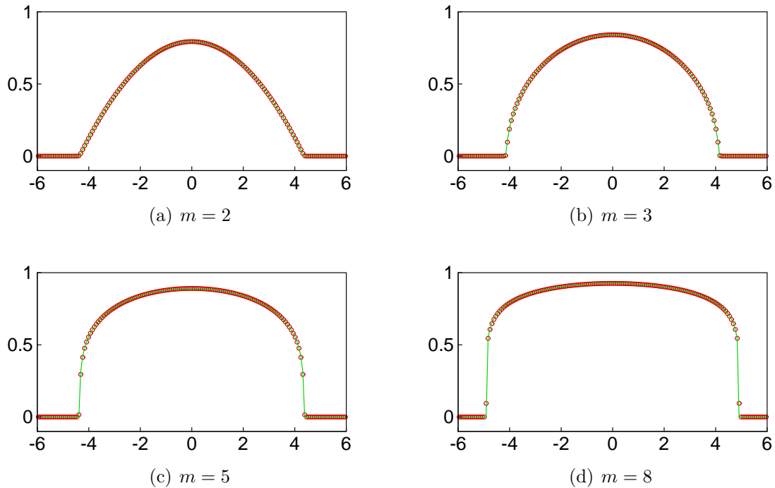
Figure 3.1: The Barenblatt solution at t = 2 . The solid line denotes the exact solution and the symbols are numerical solutions of the maximum-principle-satisfying finite volume WENO scheme.
