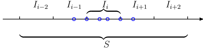
Figure 2.1: An illustration of the six points x_{i\pm\frac{1}{2}}^\alpha ( \alpha = 1, 2, 3 ).
