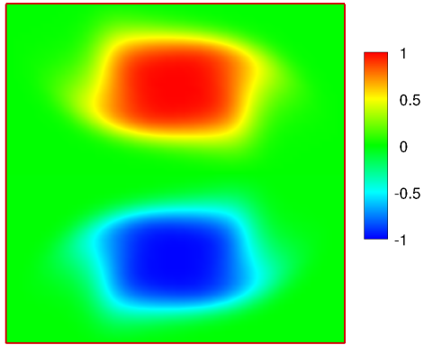
(a) 64^2 mesh
