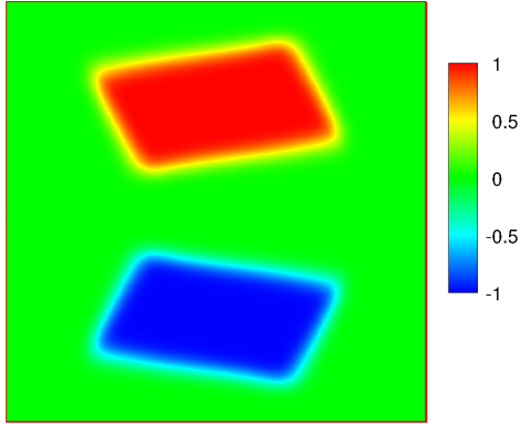
(c) 128^2 mesh
