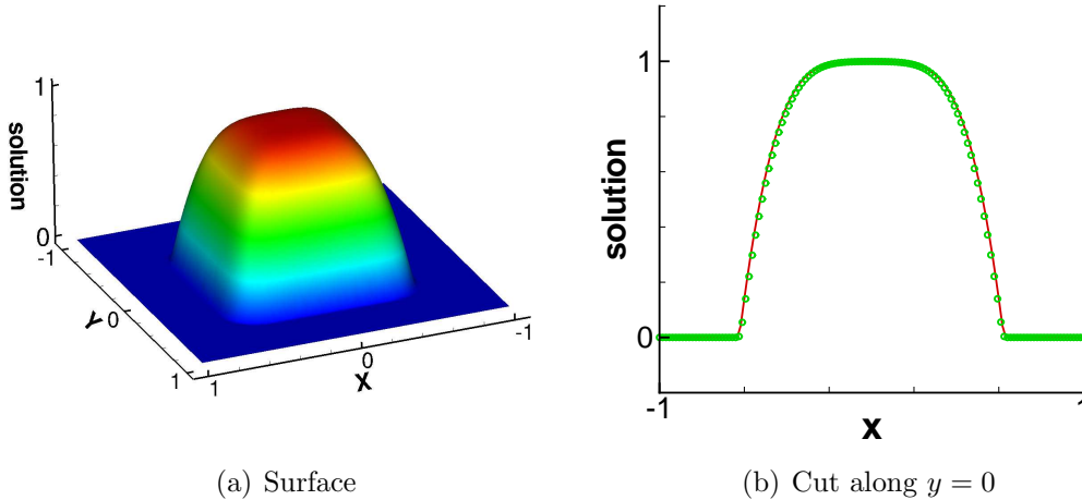
Figure 4.1: The surface on the left and the solid curve on the right are the numerical solutions of the maximum-principle-satisfying WENO scheme on a 128^2 mesh. The symbols on the right is the numerical solution of finite difference WENO scheme in [8].
