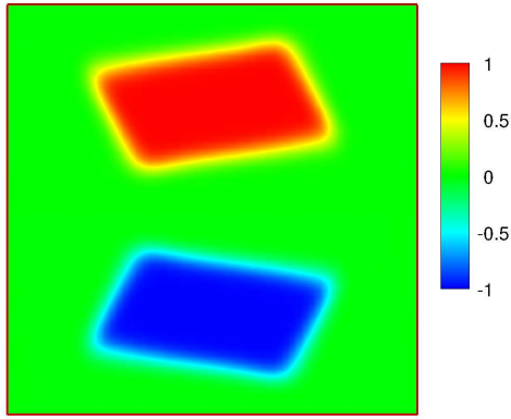
(a) 64^2 mesh
