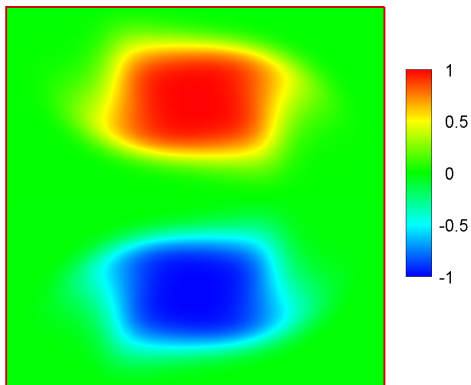
(c) 128^2 mesh
