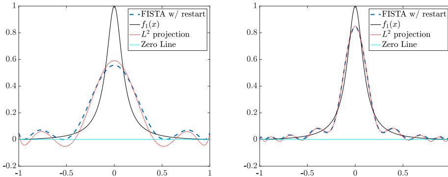
FIG. 1. The approximated polynomials for f_1(x) (4.1) with positivity constraints for n = 10 (Left), n = 20 (Right). The positive approximation is found via solving (P) by restarted FISTA on (3.4).
