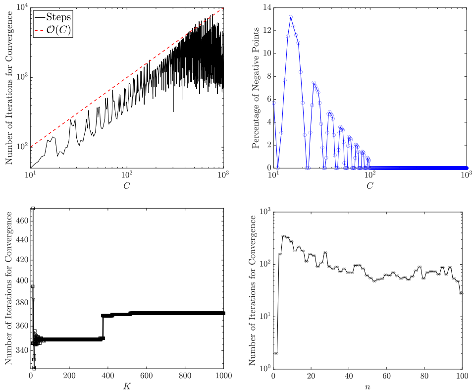
FIG. 4. The required iteration number for restarted FISTA to converge, with respect to the number of constraints C (upper left), the number of approximation samples K (lower left), and polynomial order n (lower right) for finding a positive approximation to the function f_2(x) (4.2). The percentage of negative sample points in 10^4 independent randomly tested samples with respect to C is shown in upper right.
