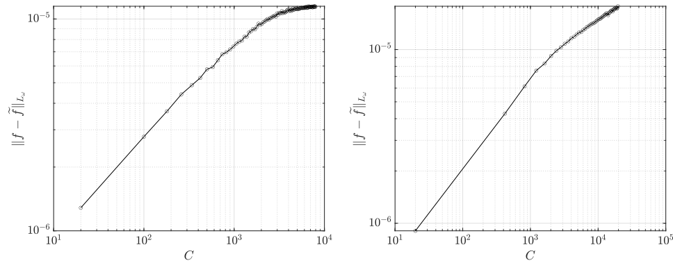
FIG. 12. The estimated approximation error (4.7) for 100-dimensional (left) and 200-dimensional (right) f_4(\mathbf{x}) (4.4) with respect to the number of constraints C using restarted FISTA when polynomial orders n = 2 . The errors are computed based on 5,000 independent randomly tested samples.
