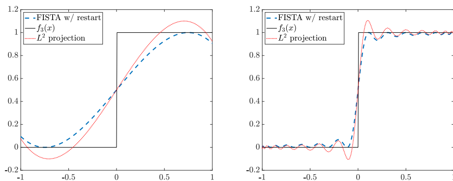
FIG. 5. The approximated polynomial for f_3(x) (4.3) with boundedness constraints for n = 5 (Left), n = 30 (Right). The bounded approximation is found via solving (\mathbf{P}) by restarted FISTA on (3.4)
