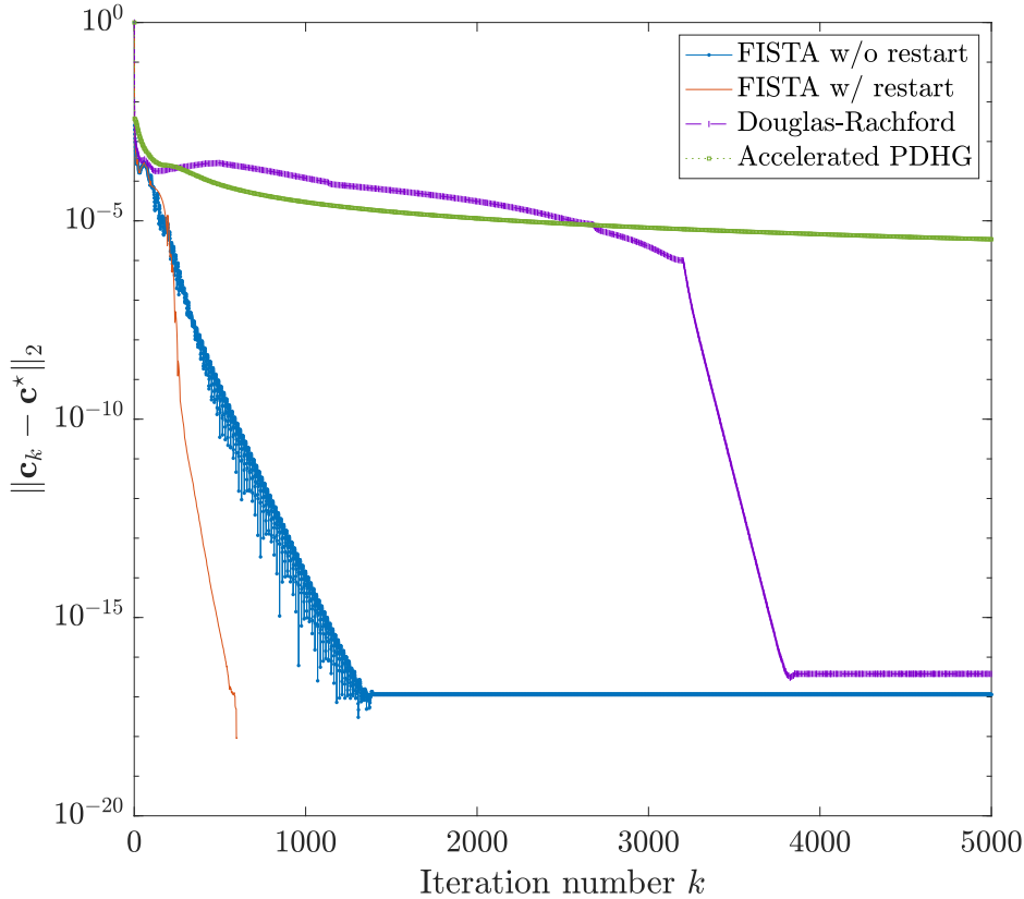
FIG. 3. The comparison of convergence curve of several methods for approximating f_2(x) (4.2) with positivity constraints when n = 20 . The reference minimizer \mathbf{c}^* is obtained numerically via restarted FISTA with 5,000 steps. For simplicity, Douglas-Rachford splitting uses the same step size as the FISTA method. We emphasize that Douglas-Rachford splitting could be much faster if tuning parameters.
