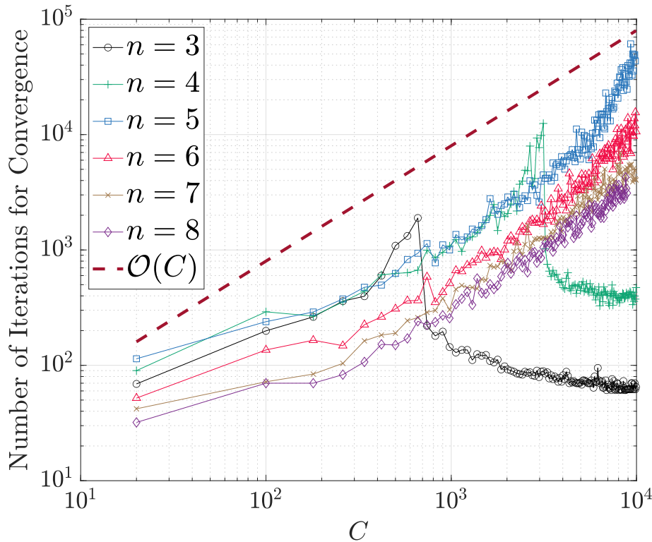
FIG. 11. The number of iterations needed for restarted FISTA to converge for 10-dimensional f_4(\mathbf{x}) (4.4) with respect to number of constraints C given polynomial order n = 3, 4, 5, 6, 7, 8 .
