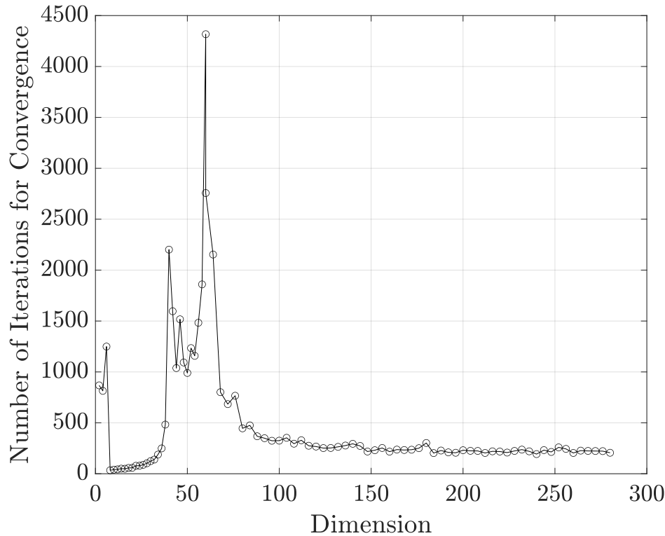
FIG. 15. The number of iterations needed for restarted FISTA to converge for f_4(\mathbf{x}) (4.4) with respect to the number of dimensions using polynomial orders n = 2 , number of approximation points N = 2,000 and number of constraints C = 2,000 .
