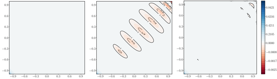
FIG. 8. The contour plots of f_6(\mathbf{x}) (4.6) (left), L^2 projection when polynomial order n = 20 (Middle) and positive approximation via solving (P) by restarted FISTA on (3.4) (Right). In these graphs, positive values are marked in blue color, negative values are marked in red. A few contour lines are drawn using black solid (zero value) and dashed (a few negative values) lines.
