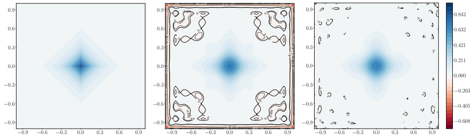
FIG. 7. The contour plot of f_5(\mathbf{x}) (4.5) (left), L^2 projection when polynomial order n = 20 (Middle) and positive approximation via solving (P) by restarted FISTA on (3.4) (Right). In these graphs, positive values are marked in blue color, negative values are marked in red. A few contour lines are drawn using black solid (zero value) and dashed (a few negative values) lines.
