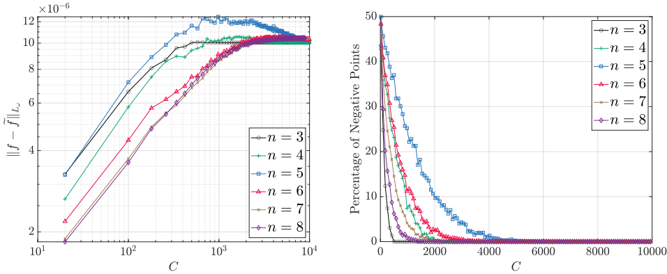
FIG. 9. Comparison of the estimated approximation error (4.7) (left) and percentage of negative sample points (right) with respect to the number of constraints C for 10-dimensional f_4(\mathbf{x}) (4.4) using restarted FISTA at polynomial orders n = 3, 4, 5, 6, 7, 8 . These quantities are computed based on 5,000 independent randomly tested samples.
