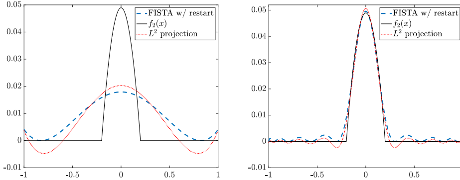
FIG. 2. The approximated polynomials for f_2(x) (4.2) with positivity constraints for n = 5 (Left), n = 20 (Right). The positive approximation is found via solving (P) by restarted FISTA on (3.4).
