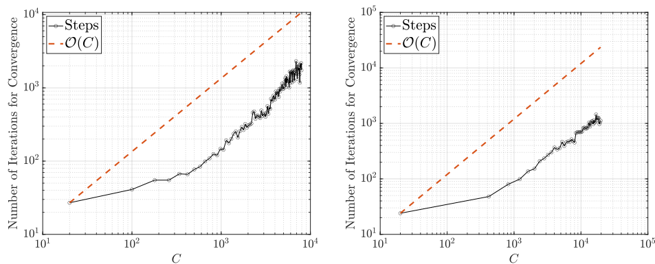
FIG. 14. The number of iterations needed for restarted FISTA to converge for 100-dimensional (left) and 200-dimensional (right) f_4(\mathbf{x}) (4.4) with respect to the number of constraints C when polynomial orders n = 2 .
