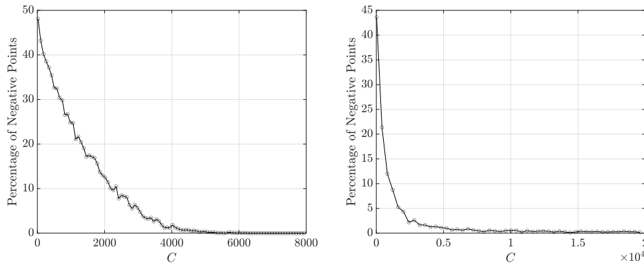
FIG. 13. The percentage of negative sample test points of restarted FISTA method (based on 5,000 independent randomly tested samples) for 100-dimensional (left) and 200-dimensional (right) f_4(\mathbf{x}) (4.4) with respect to the number of constraints C when polynomial orders n = 2 .
