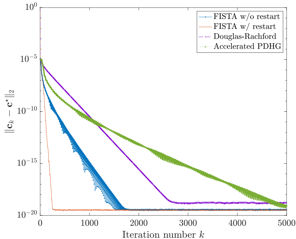
FIG. 10. The comparison of convergence curve of several methods for approximating 10 dimensional f_4(\mathbf{x}) (4.4) with positivity constraints when n = 3 . The reference minimizer \mathbf{c}^* is obtained numerically via restarted FISTA with 5000 steps. For simplicity, Douglas-Rachford splitting uses the same step size as the FISTA method. We emphasize that Douglas-Rachford splitting could be much faster if tuning parameters.
