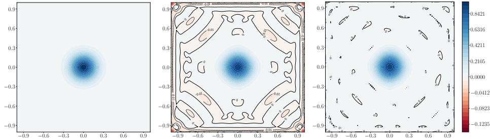
FIG. 6. The contour plots of f_4(\mathbf{x}) (4.4) (left), L^2 projection when polynomial order n = 20 (Middle) and positive approximation via solving (P) by restarted FISTA on (3.4) (Right). In these graphs, positive values are marked in blue color, negative values are marked in red. A few contour lines are drawn using black solid (zero value) and dashed (a few negative values) lines.
