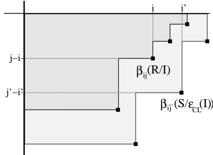
FIGURE 1. The Betti diagrams of R/I and S/\epsilon_{\text{CL}}(I) , and their extremal Betti numbers.
