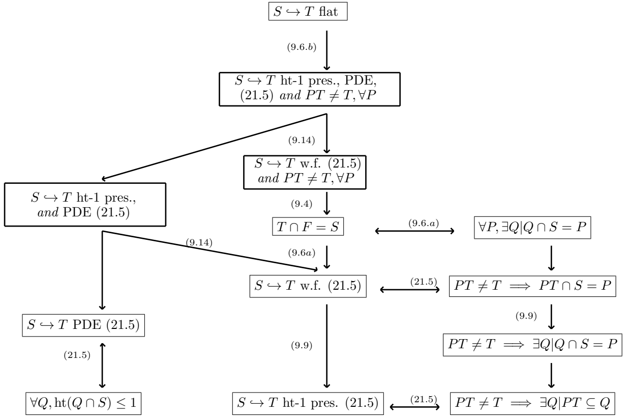
Diagram 21.9.0. The relationships among properties of an extension S \hookrightarrow T of Krull domains.
