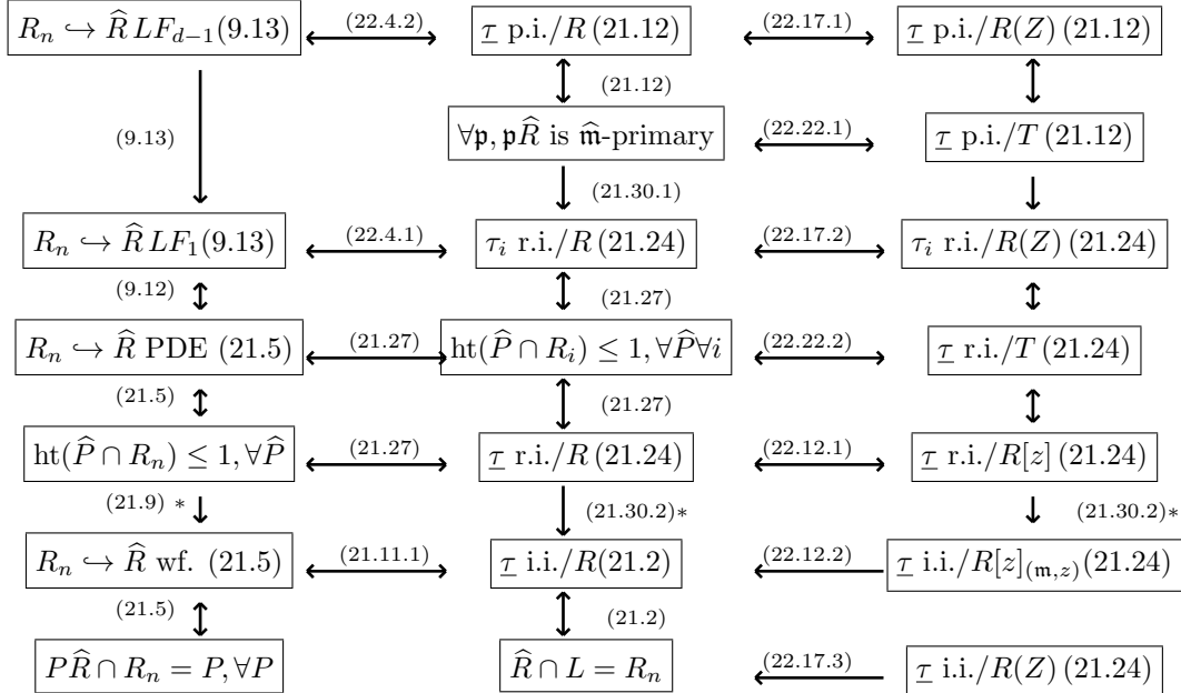
Diagram 22.26.0 Implications among the properties.
