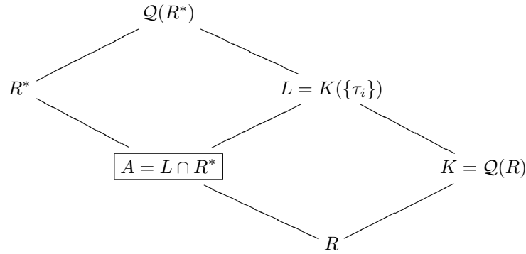
Diagram 5.3.1. A := L \cap R^*
