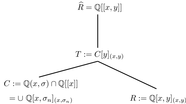
Diagram 12.17.a. The rings of the example
