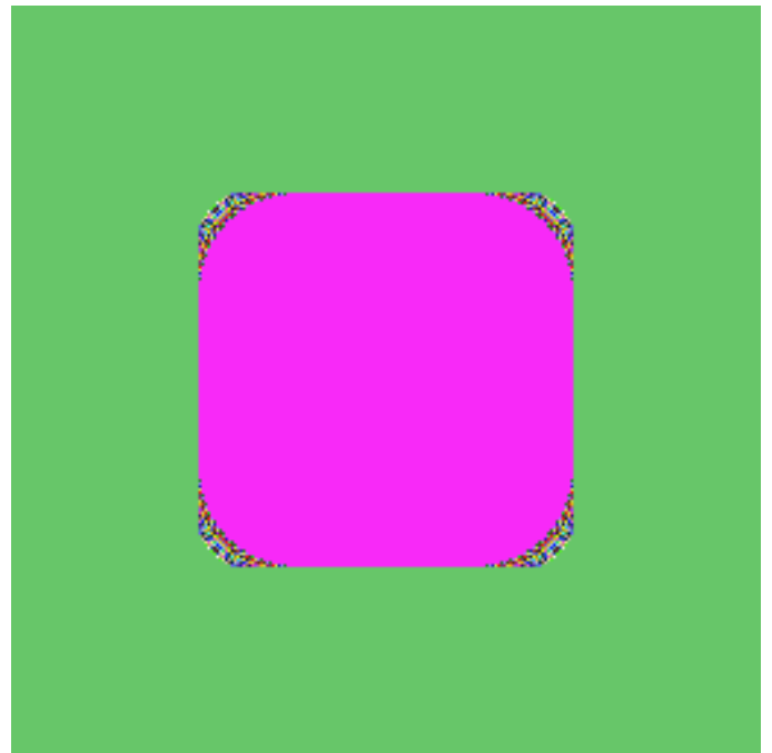
FIGURE 11. The projection onto a 256 \times 256 grid of the exact solution of the continuous BV problem, in “false color”.
