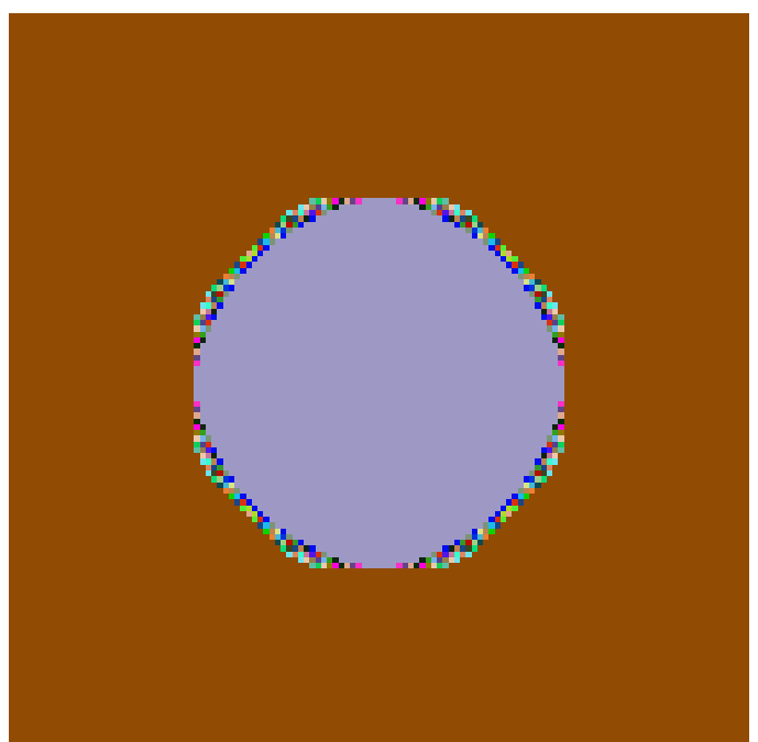
FIGURE 4. The solution of the discrete BV problem using the upwind definition (17) in “false color”.
