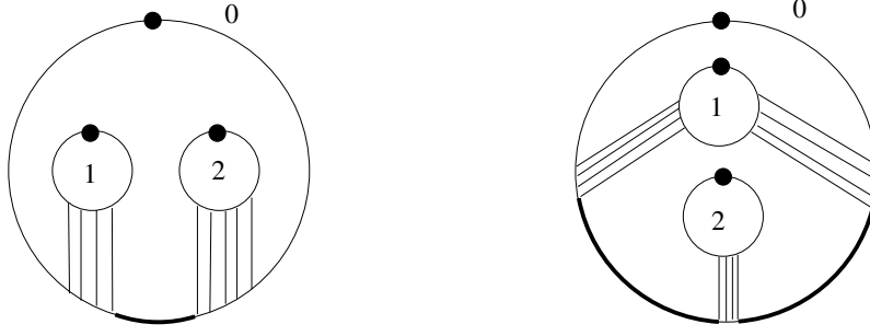
Figure 22. Examples of the partitioned families yielding \cup , \circ_i in the string topology/Deligne setting and \sqcup and \sqcup_i in the moduli setting. The outer angles are the ones with the dot, the bold angles are the non-partitioning inner angles are marked in bold.
