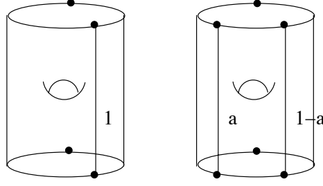
Figure 16. The two basic unstable arc graphs G and H_a .
