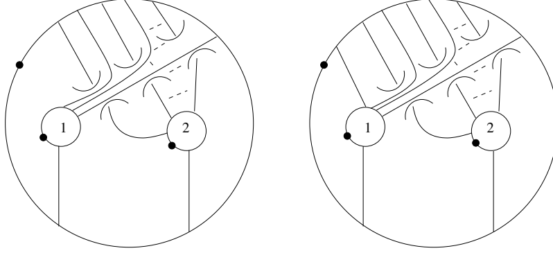
Figure 17. The \cup_i operations for i even and i odd, These are also the cells for upper hemispheres of S^\infty in its hemispherical decomposition.
