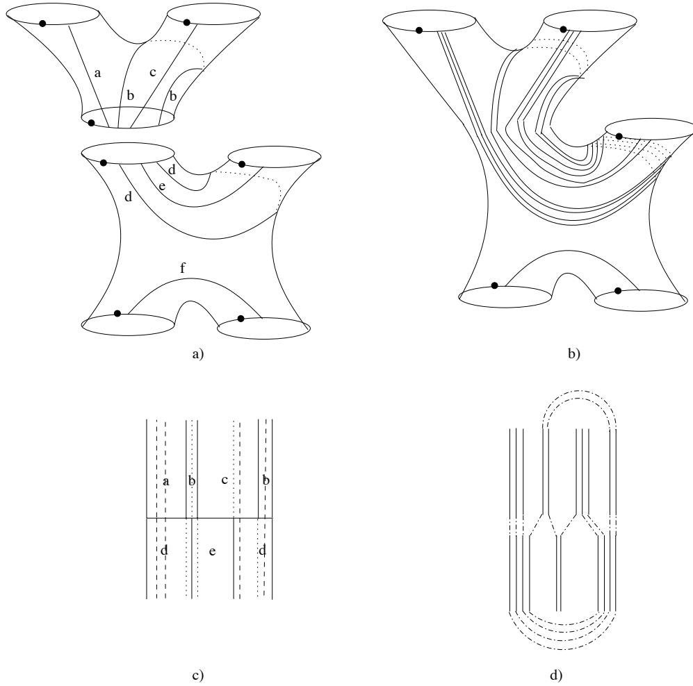
Figure 5. a) The arc graphs which are to be glued assuming the relative weights a, b, c, d and e as indicated by the solid lines in c). b) The result of the gluing (the weights are according to c). c) The combinatorics of cutting the bands. The solid lines are the original boundaries, the dotted lines are the first cuts, and the dashed lines represent the recursive cuts. d) The combinatorics of splitting and joining flags.
