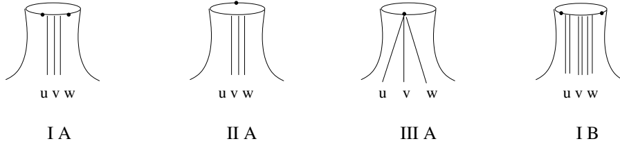
Figure 1. I A. Arcs running to a point on the boundary; II A. Arcs running to a point at infinity; III A. Arcs in a window; I B. Bands in a window
