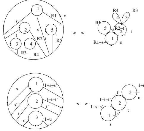
Figure 7. A Cactus and a spineless Cactus
