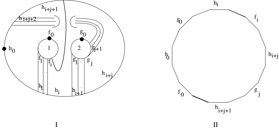
Figure 21. A partitioned arc graph with decorations by elements of A and one of its decorated polygons. The bold line corresponds to the bold edge.
