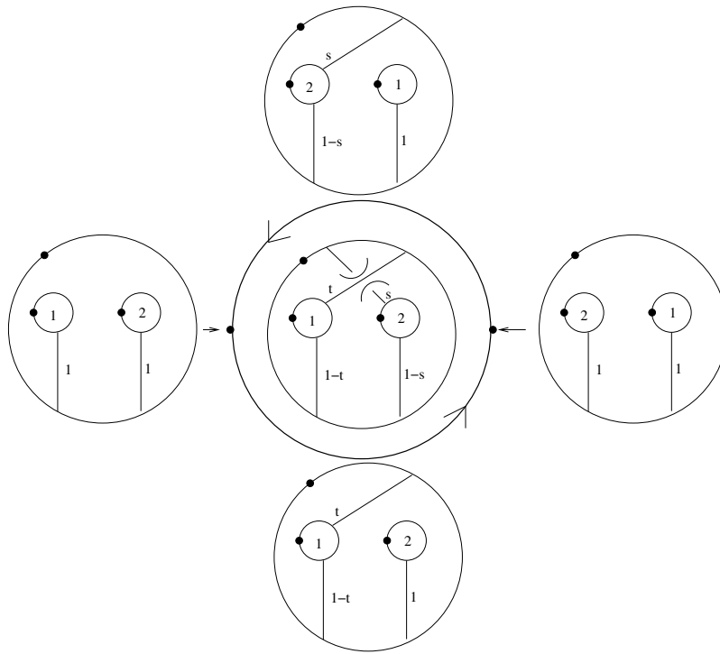
Figure 19. The \cup_2 operation after stabilization
