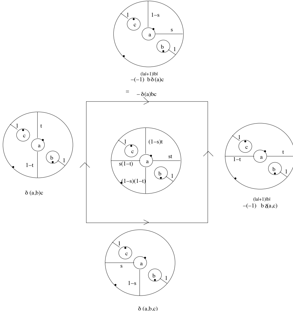
Figure 10. The basic chain homotopy responsible for BV
