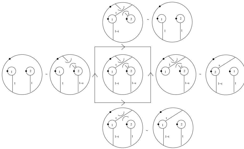
Figure 18. The \cup_2 operation and its boundary before stabilization and stable representatives of the boundary components
