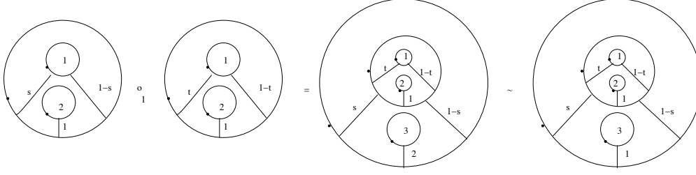
Figure 12. The first iterated gluing of *
