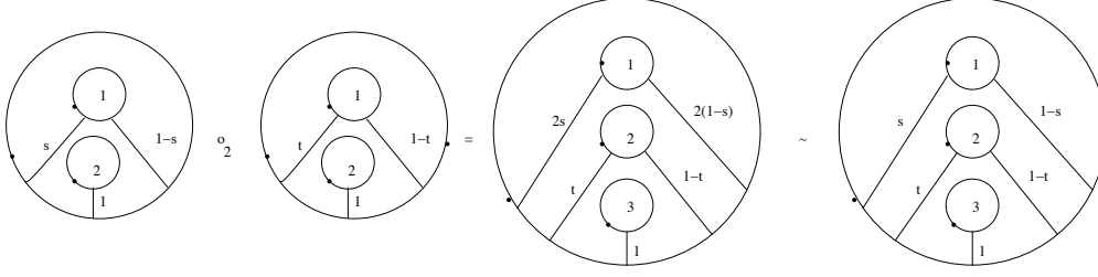
Figure 15. The other iteration of *
