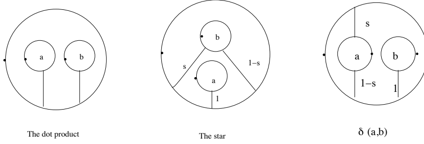
Figure 8. The binary operations
