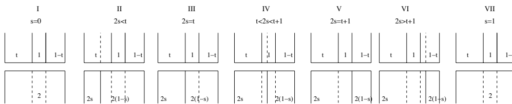
Figure 14. The different cases of gluing the bands
