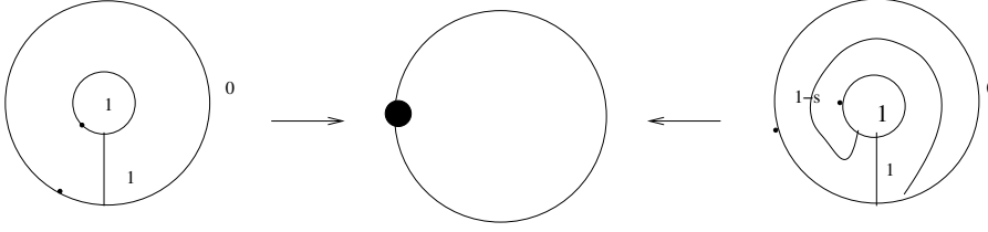
Figure 4. The CW complex A_{0,2}^0 = S^1 . We indicated the base point and a generic element
