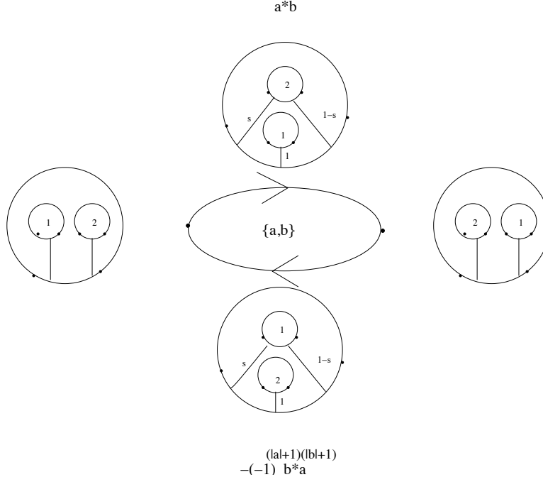
Figure 9. The definition of the Gerstenhaber bracket
