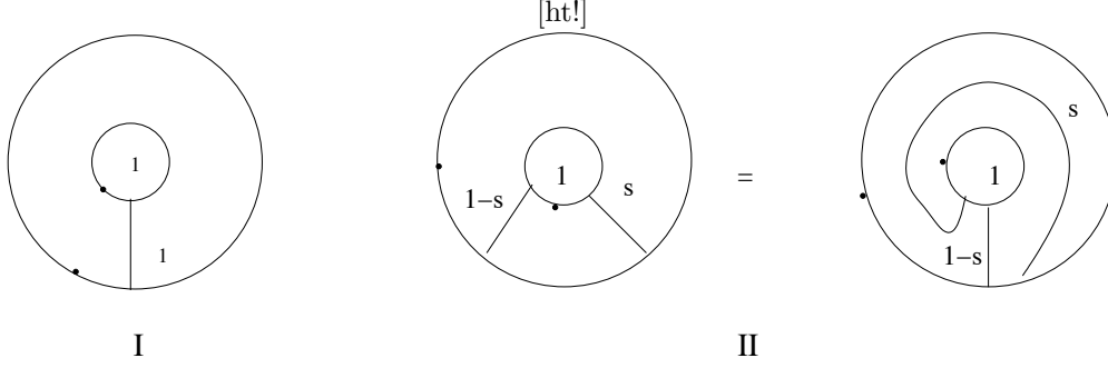
Figure 6. I, the identity and II, the arc family \delta yielding the BV operator
