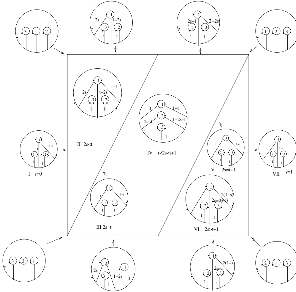
Figure 13. The glued family after normalization
