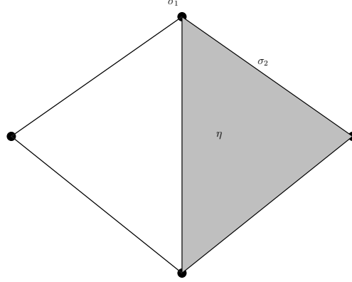
FIGURE 2. The complex \Delta_{\mathcal{Q}} .
