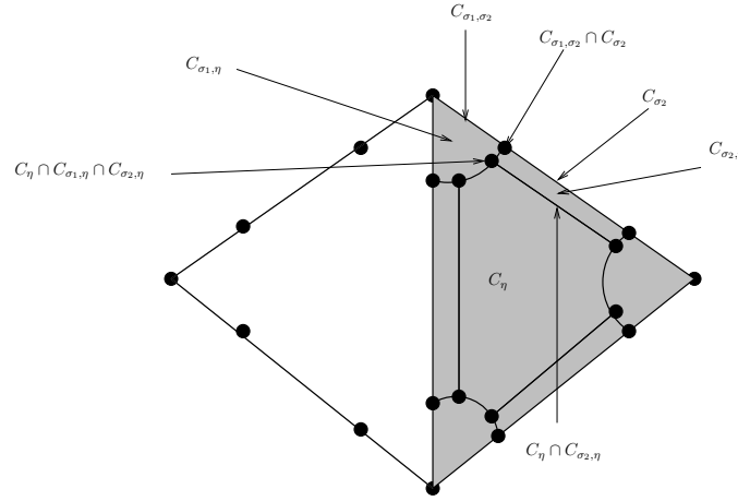
FIGURE 3. The corresponding complex \mathcal{C}(\Delta_{\mathcal{Q}}) .
