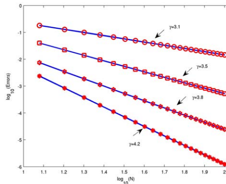
FIGURE 4.2. H^3 -Errors against various N in log-log scale for Example 2 with several \gamma .
