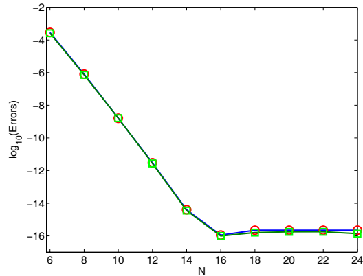
FIGURE 4.1. the maximum pointwise error (marker “o”) and the L^2 -error (marker “□”) against various N in semi-log scale for Example 1.
