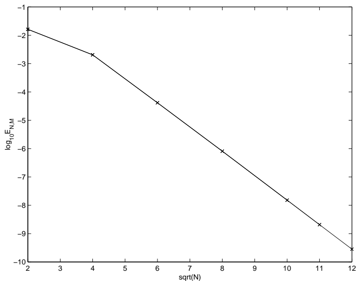
FIGURE 5.1. Convergence rate for N = M^2
