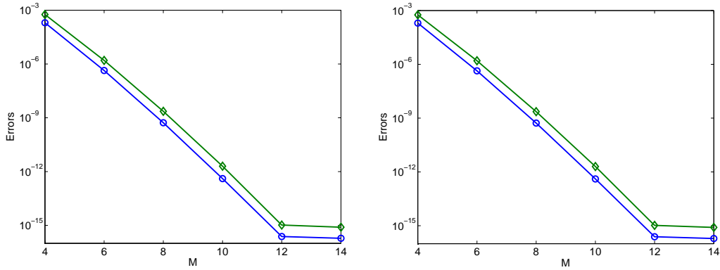
FIGURE 5.2. Maximum pointwise errors (marked by ' \diamond ') and L^2 -errors (marked by ' \circ ') against various degree M for Example 2. Left: function \gamma = 0 ; Right: function \gamma = 1 .
