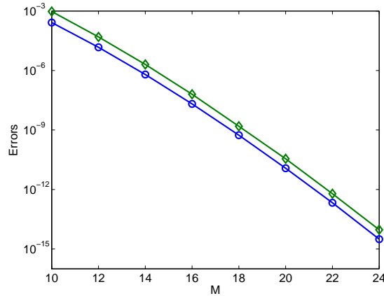
FIGURE 5.3. Maximum pointwise errors (marked by ' \diamond ') and L^2 -errors (marked by ' \circ ') against various degree M for Example 3.
