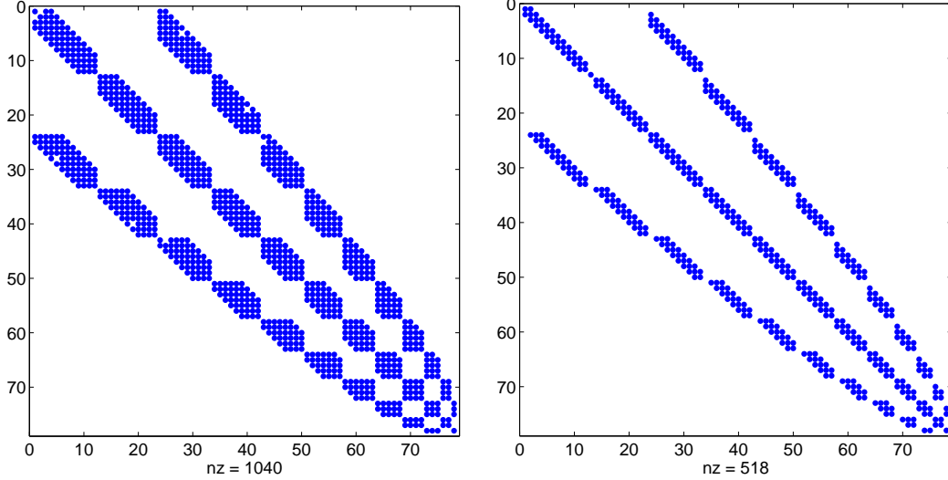
FIGURE 4.1. Structure of the mass matrix A (left) and the stiff matrix B (right) with M = 14 : nz is the number of non-zero elements.
