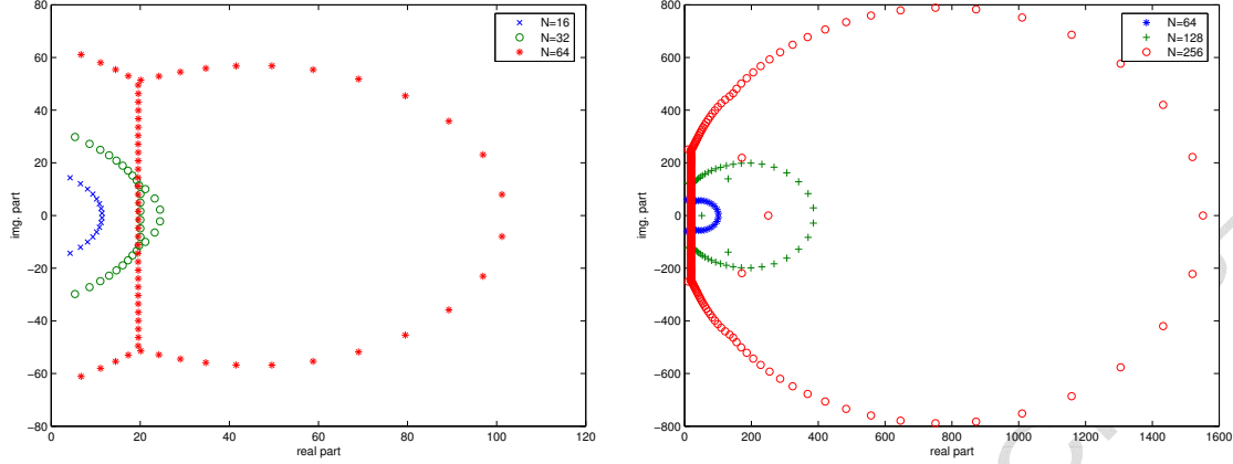
FIGURE 1. eigenvalue distribution of W^{-1}S with a(x) = 1 .
