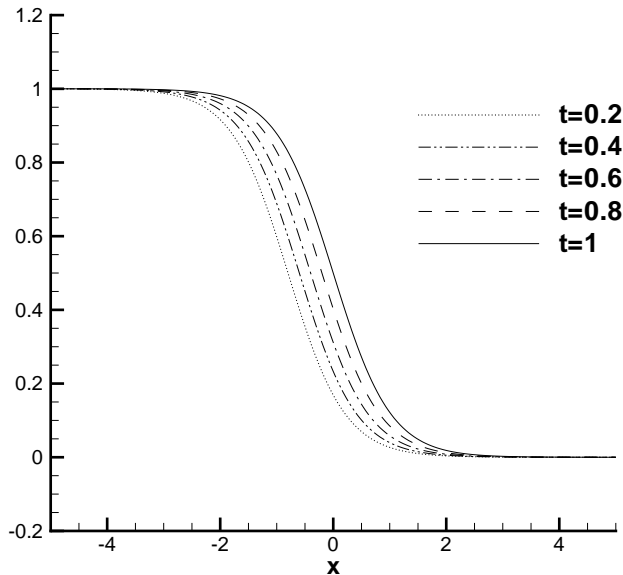
FIG. 5.10. Time evolution of the mean solution with the initial condition (5.5).
