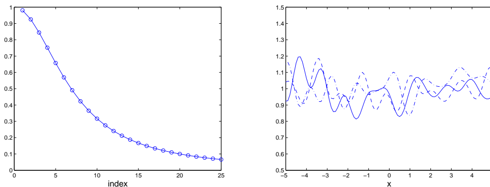
FIG. 5.9. Construction of the random diffusivity field (5.4) with correlation length 0.5. Left: eigenvalues of Karhunen-Loève expansion. Right: sample realizations of the diffusivity field with N = 20 .
