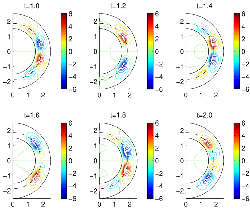
Fig. 2. R_m = 100 . Contours of the azimuthal field B_\phi in a meridional plane at different time.
