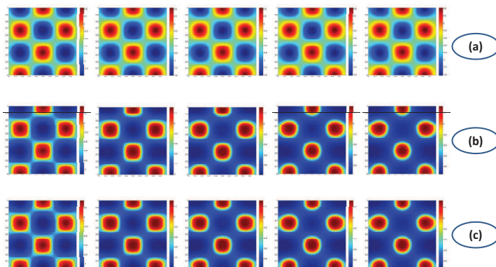
Figure 6: The phase portrait of the binary fluid mixing with the Flory-Huggins energy for all three models at t=0.1,0.2,0.3,0.4,0.5 . (a) M1, (b) M2, (c) M3.
