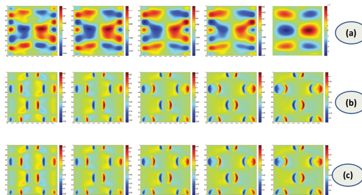
Figure 11: The velocity component u at t=0.1,0.2,0.3,0.4,15 in the case of binary fluid mixing for all three models. (a) M1 , (b) M2 , (c) M3 . The solutions nearly reach quasi-steady state at t=15 .
