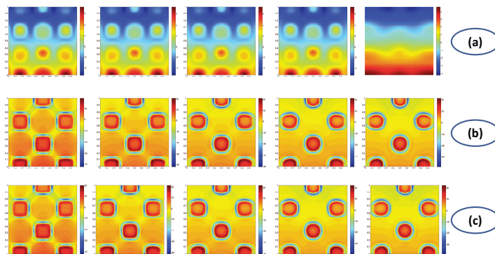
Figure 13: The hydrodynamic pressure p at t=0.1, 0.2, 0.3, 0.4, 15 in the case of binary fluid mixing for all three models. (a) M1, (b) M2, (c) M3. The solutions nearly reach quasi-steady state at t=15 .
