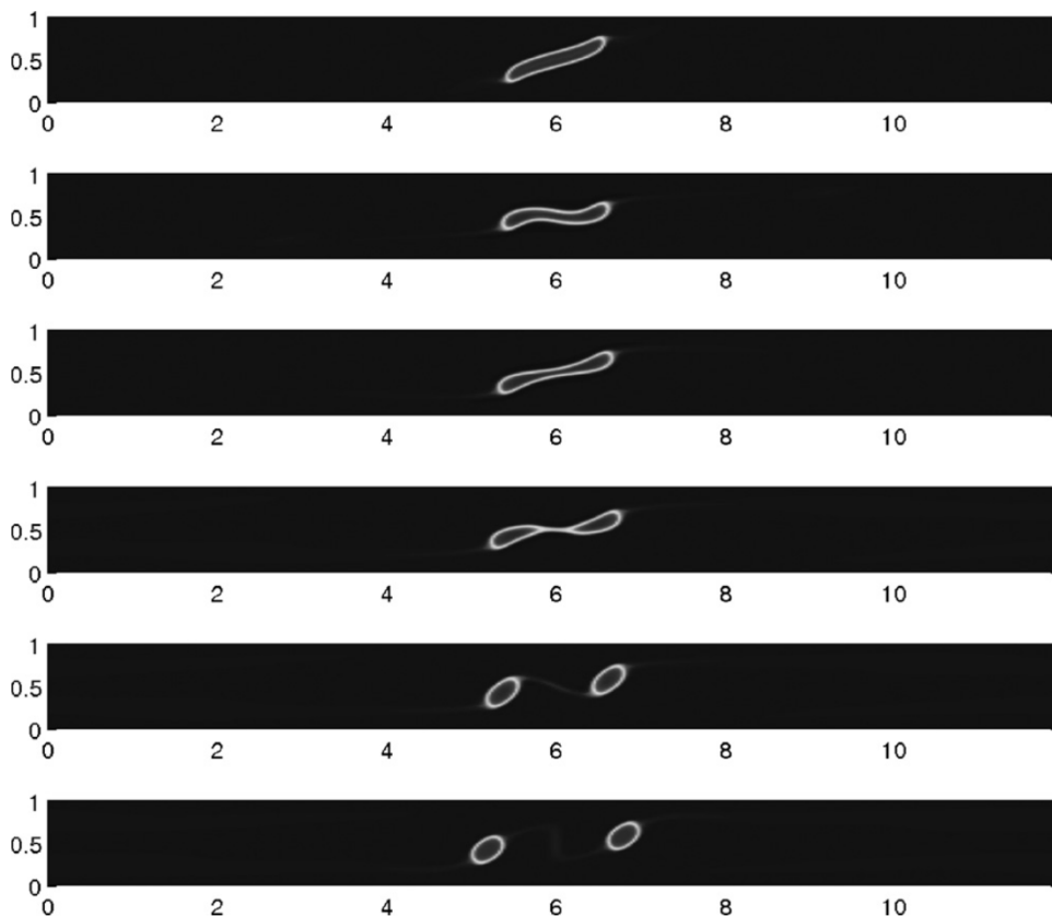
Newtonian drop that is immersed in a Newtonian fluid, at t=0.1, 0.4, 0.7, 0.9, 1, 1.1 with shear rate \kappa=15 with domain size
