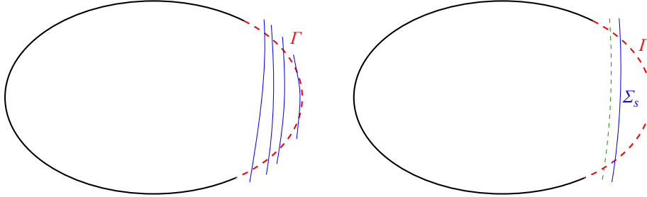
FIGURE 3. An illustration to Theorem 2.3 and its proof. Left: the family \Sigma_s . Right: The “inductive” step of the proof. The curve on the right is \Sigma_s ; the dashed one on left is at distance \epsilon from \Sigma_s .
