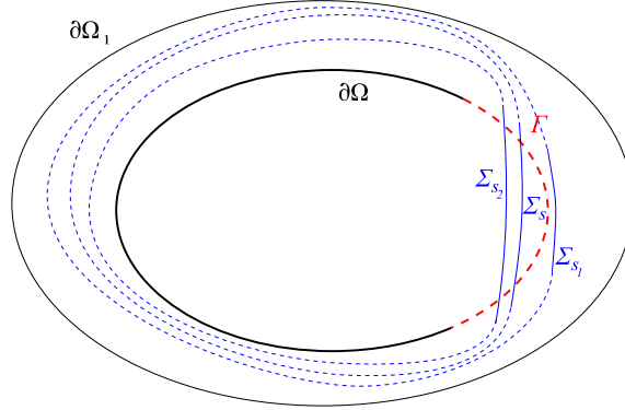
FIGURE 2. A typical example of the family \Sigma_s . The surfaces \Sigma_s do not need to be closed, and the dashed parts shows how they can be extended to closed surfaces. For each \Sigma_s , \Sigma_s^{\text{int}} is the interior, while \Sigma_s^{\text{ext}} is the exterior of the surface.
