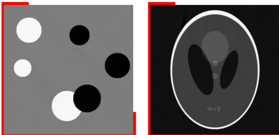
Figure 5. Partial data inversion with data on the indicated part of \partial\Omega . Neumann series inversion with 10 terms, T=5 , on the square [-1,1]^2 . Left: constant speed c=1 , L^2 error =0.7%. Right: variable c=1+0.3\sin(\pi x^1)+0.2\cos(\pi x^2) , L^2 error =2%. We average with \phi as in remark 2, i.e., with weight \chi=1 in [0, T] , see (20). Again, the most visible artifacts can be explained by the presence of corners.
