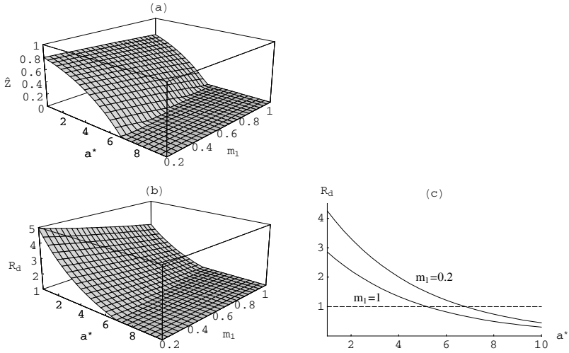
FIGURE 1. (a) is a plot of the fraction of occupied patches \hat{Z} versus the critical age of colonization a^* and extinction rate of young patches m_1 . (b) and (c) illustrate how the reproductive number \mathcal{R}_d changes with a^* and m_1 .
