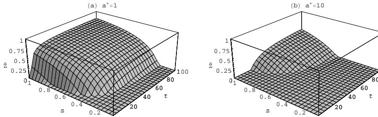
FIGURE 2. Plots of the fraction of occupied patches \widehat{Z} versus the expected fraction of suitable habitat \bar{s} and the expected patch life time \bar{\tau} for different values of the critical age of colonization a^* .
