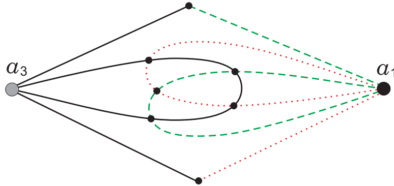
Figure 8: Pseudo-diagonal connecting corners a_1 and a_3 of \mathcal{Q} .
