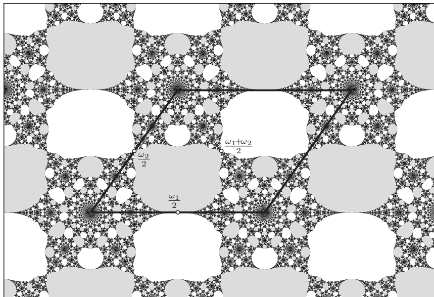
FIGURE 3. Julia set corresponding to \tau = 1/2 + ib_1 .
