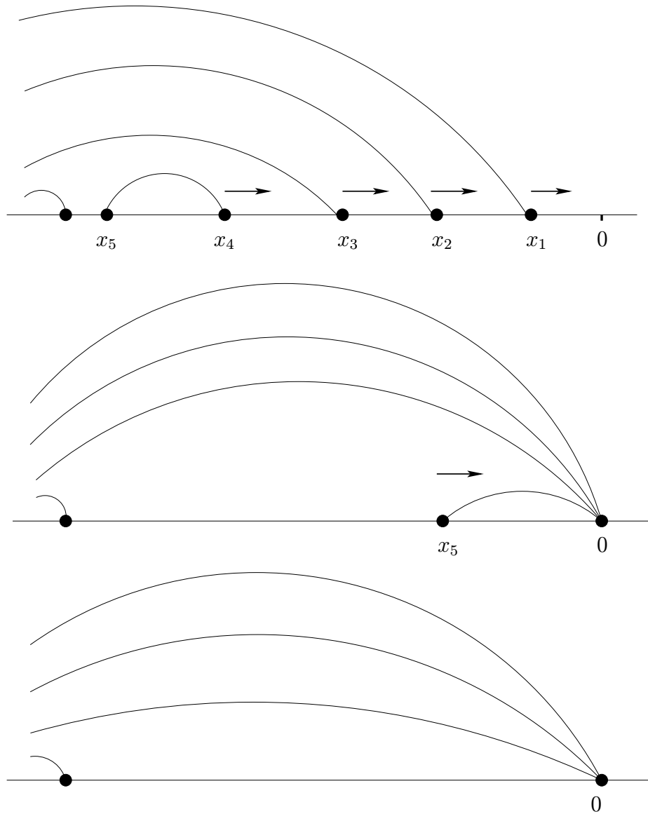
Fig. 3. Steps of collapse. Case 2 occurs on the 5-th step with k = 5 .
