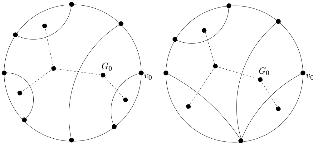
Fig. 2. Collapse of a net. The trees S are shown in dotted lines.
