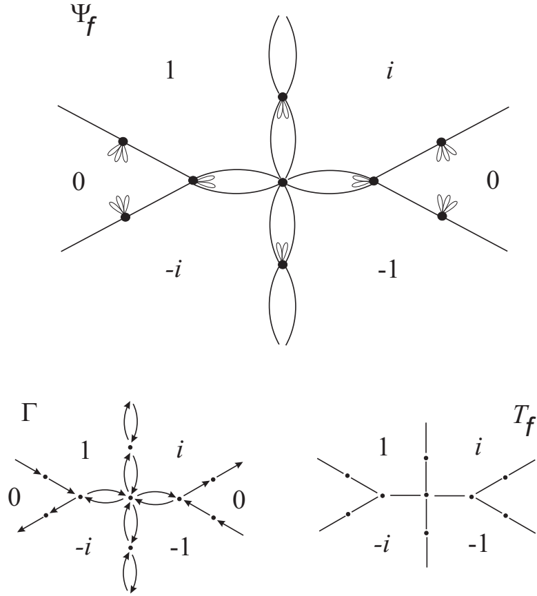
Fig 3. Cell decomposition \Psi_f .
