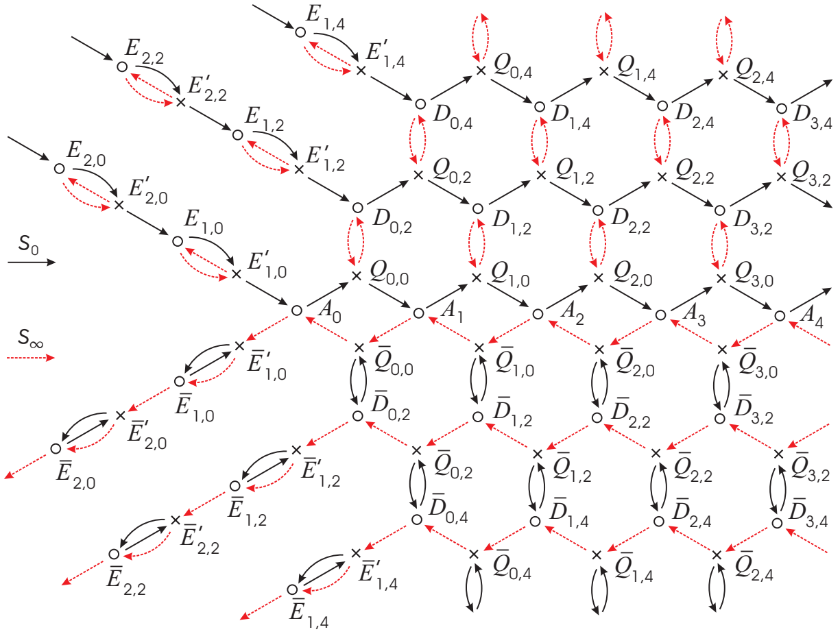
Fig 10. Monodromy action on the even part of G .
