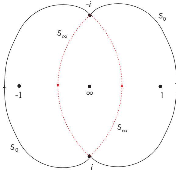
Fig 6. Paths s_0 and s_\infty used in the deformation of \Psi_0 .
