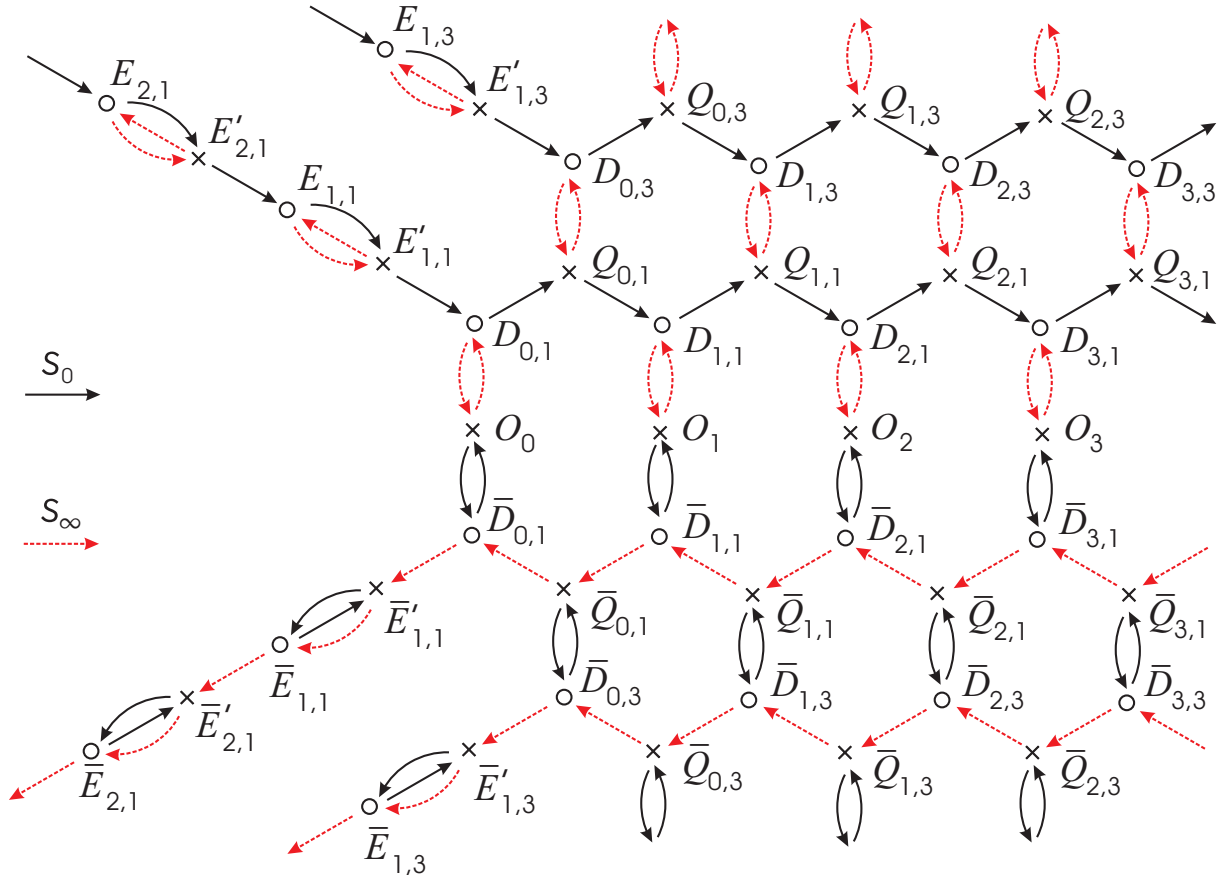
Fig 11. Monodromy action on the odd part of G .
