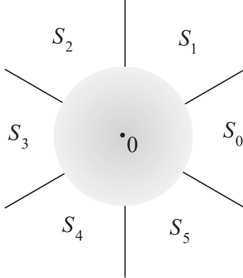
Fig 1. Stokes sectors
