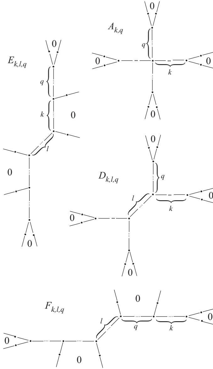
Fig S2. Classification of QES sextic trees
