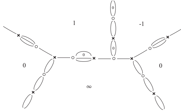
Fig C9. Line complex of type A_{1,0}
