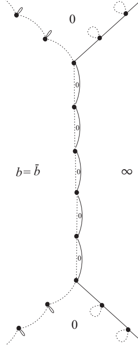
FIGURE 11. The limit cell decomposition of Fig. 8 as b \rightarrow -1 (solid and dotted lines).
