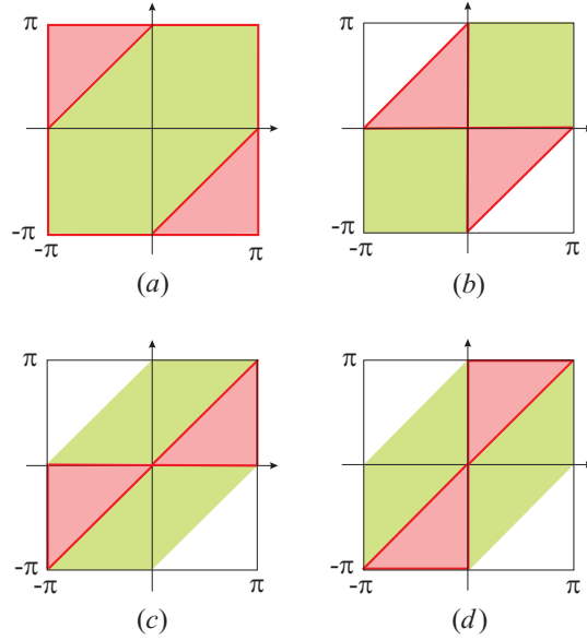
FIGURE 3. The values of (\arg t, \arg c) in Example 3.5 where both \mathbf{R}_+ and \mathbf{R}_- are good (light shaded) and where \mathbf{R}_- is not good (dark shaded). (a) d and m even; (b) d and m odd; (c) d even, m odd; (d) d odd, m even.
