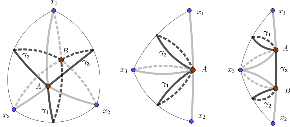
Figure 2: Three types of spheres
