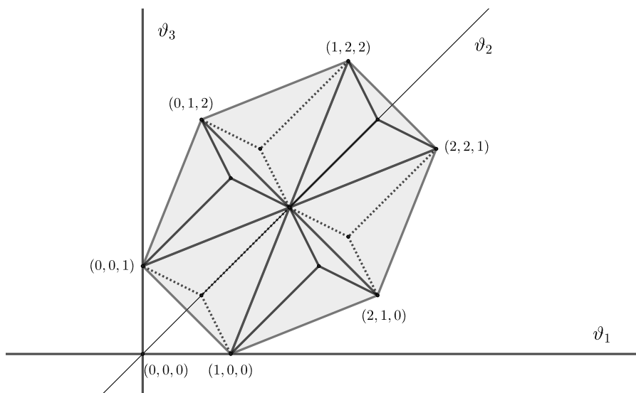
Figure 7: Angle vectors of spherical triangles
