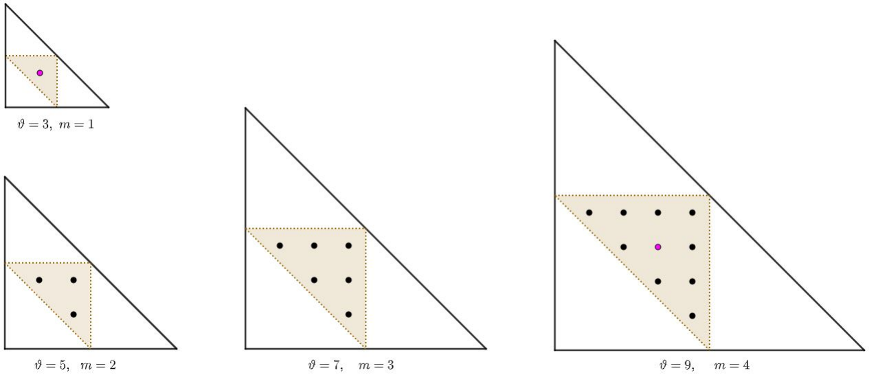
Figure 11: Angle carpets for \vartheta = 2m + 1 odd integer.
