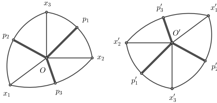
Figure 6: Two isomorphic triangles \Delta and \Delta'
