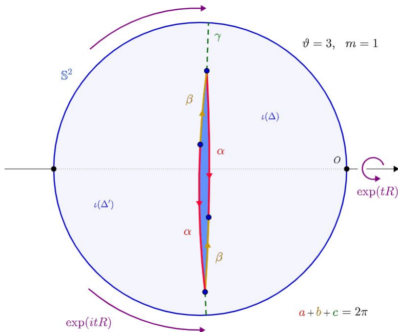
Figure 12: The developing map \iota for T(\Delta) \setminus (\alpha \cup \beta) , where \Delta is a triangle with \vartheta = 3 and edges \alpha, \beta, \gamma of lengths a, b, c . The two congruent triangles \Delta, \Delta' are mapped to antipodal hemispheres, and their edges are mapped to the separating equator.
