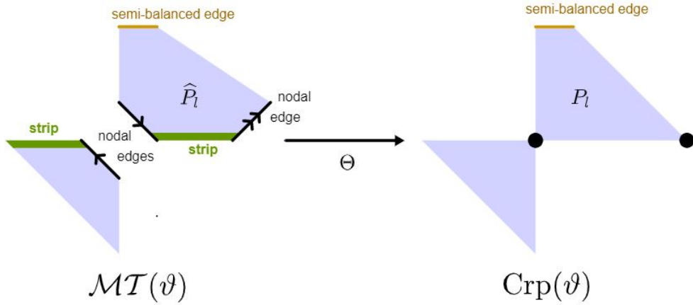
Figure 10: The map \Theta . Unmarked edges are ideal edges.
