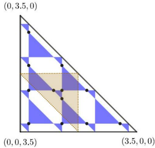
Figure 8: The angle carpet \text{Crp}(\frac{7}{2}) , composed of 16 open triangles and 12 nodes. The shaded area represents points in \text{Bal}(\vartheta) .
