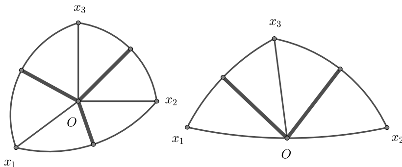
Figure 3: Voronoi graphs of balanced triangles
