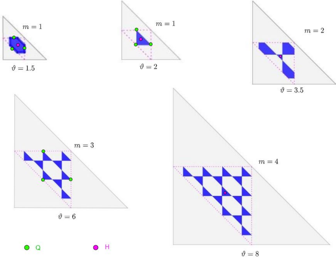
Figure 9: Balanced carpets for \vartheta = 1.5, 2, 3.5, 6, 8 .
