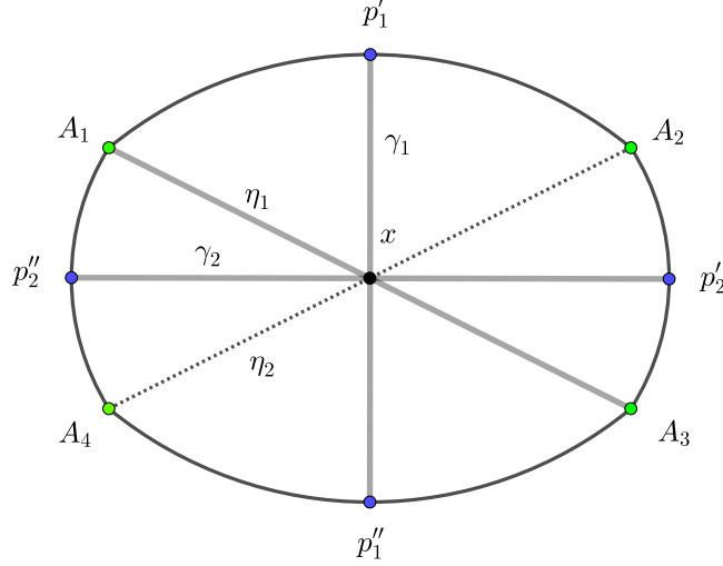
Figure 5: Eight graph case
