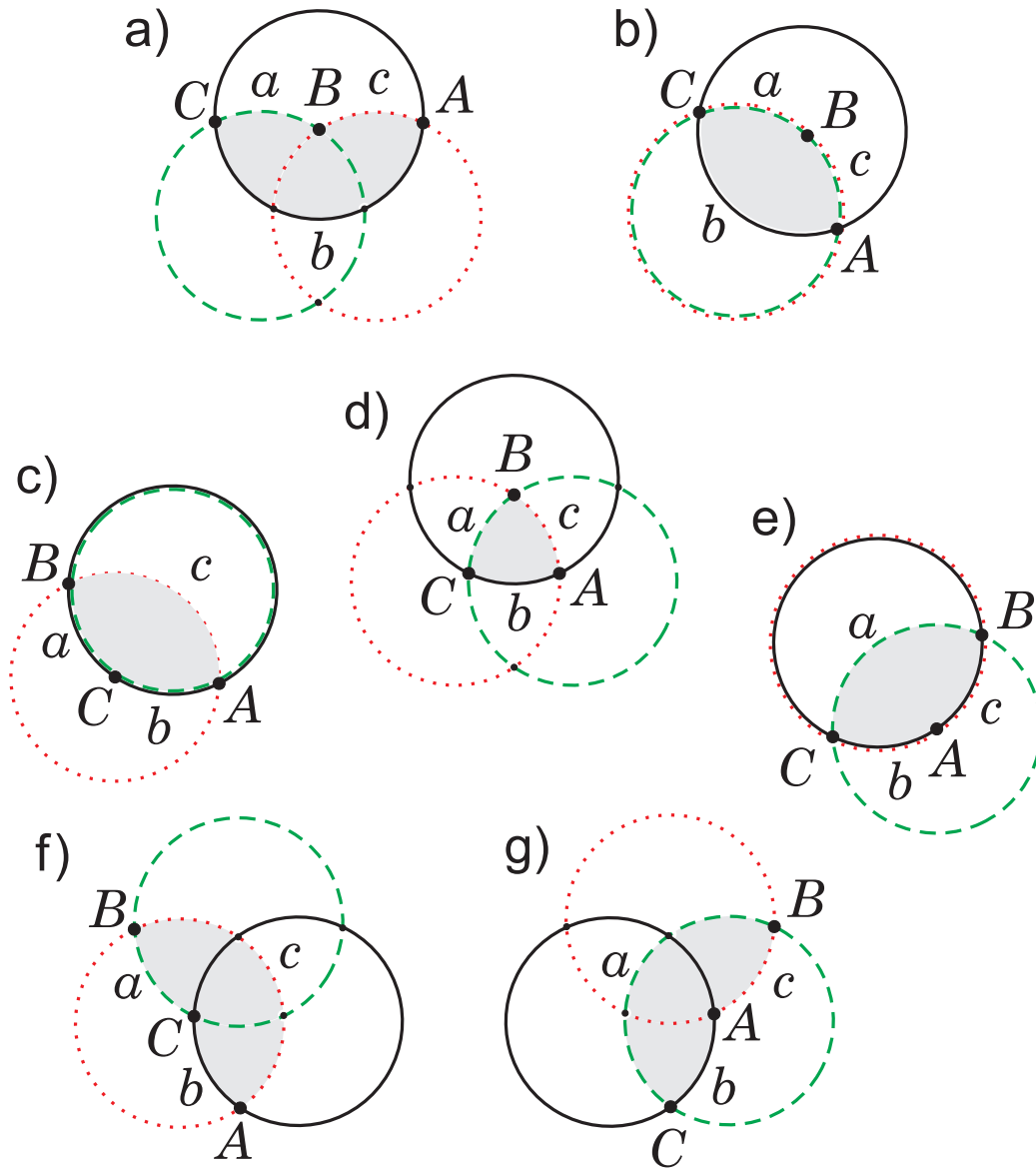
Figure 6: Triangles with A + B + C < 3 in a neighborhood U of the vertex (1, 1, 1) . When two sides of a triangle are mapped to the same circle, that circle is shown in dual color/style.
