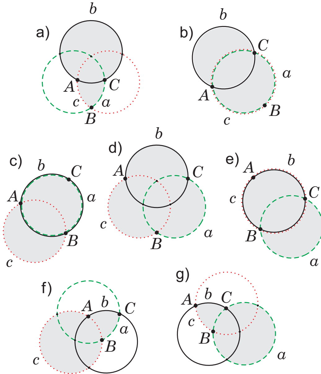
Figure 5: Triangles with A + B + C > 3 in a neighborhood U of the vertex (1, 1, 1) . When two sides of a triangle are mapped to the same circle, that circle is shown in dual color/style.
