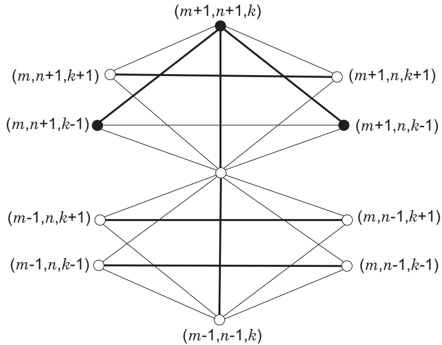
Figure 4: Tetrahedra adjacent to edges in X_1 of the second type meeting at a marginally unbalanced vertex (m, n, k) with m+n = k-1 . Balanced vertices are shown as black dots.
