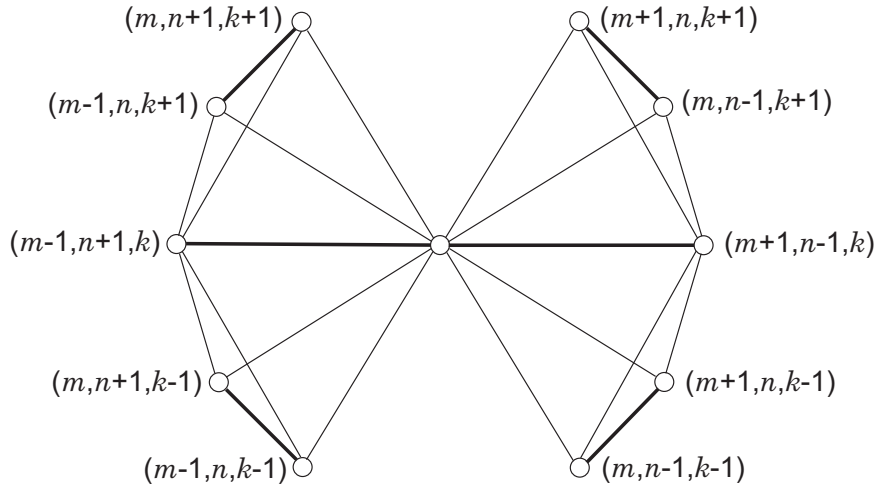
Figure 1: Tetrahedra adjacent to edges in X_1 of the first type meeting at a vertex (m, n, k) with m + n < k - 1 . Edges in X_1 are shown in bold line.
