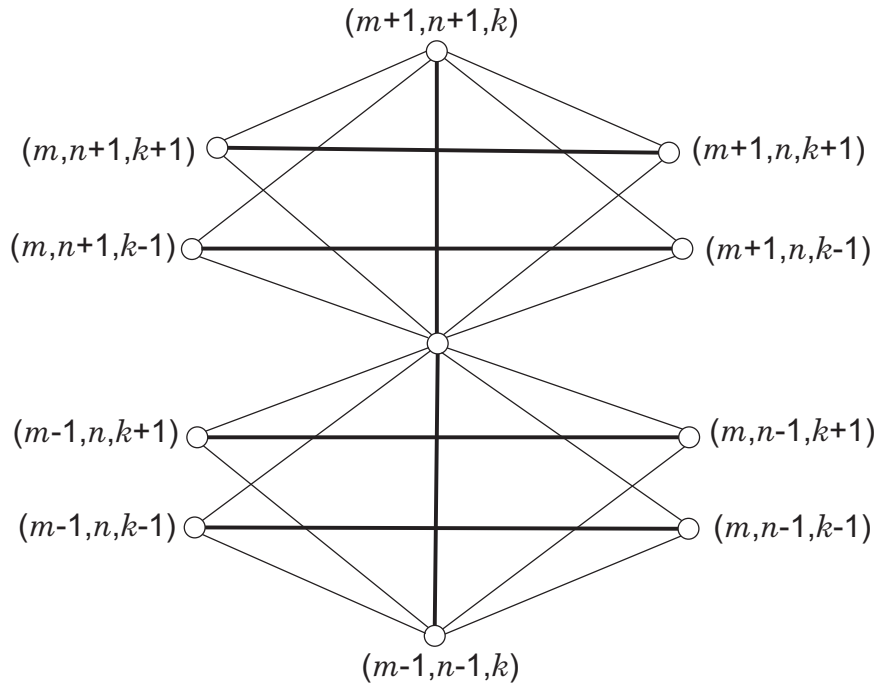
Figure 2: Tetrahedra adjacent to edges in X_1 of the second type meeting at a vertex (m, n, k) with m + n < k - 1 . Edges in X_1 are shown in bold line.
