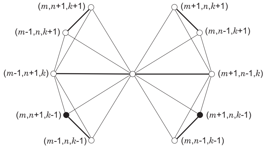
Figure 3: Tetrahedra adjacent to edges in X_1 of the first type meeting at a marginally unbalanced vertex (m, n, k) with m+n = k-1 . Balanced vertices are shown as black dots.
