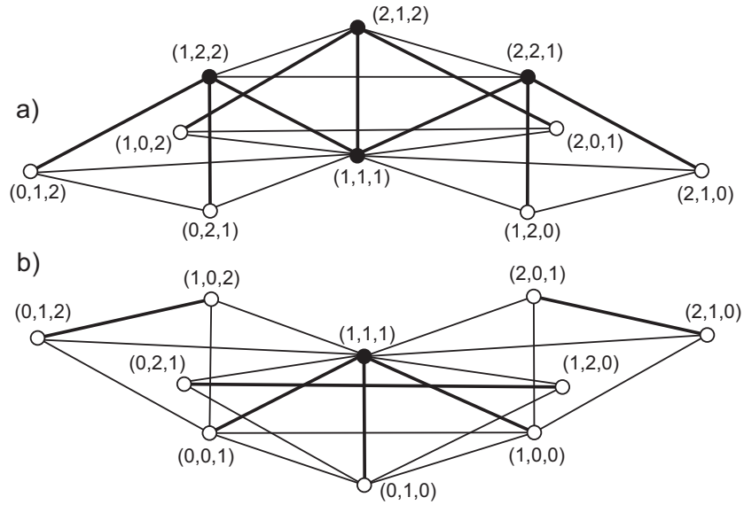
Figure 7: The upward (a) and downward (b) tetrahedra adjacent to the vertex (1, 1, 1) in Lemma 4.1. Edges in X_1 are shown in bold line.
