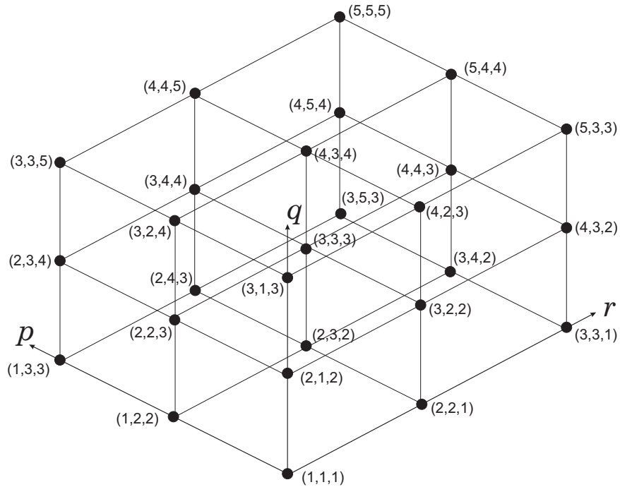
Figure 8: The sets \Lambda_0 and \Lambda_1 of balanced vertices and edges in \mathbb{R}^3_{p,q,r} .
