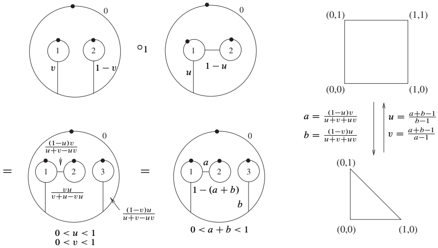
Figure 4. A gluing in \mathcal{C}_o^*(\mathcal{A}rc) together with a reparameterization of (0, 1) \times (0, 1) to the inside of the 2-simplex.
