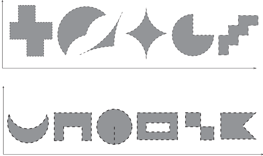
FIGURE 1. Top: examples of semi-monotone subsets of the plane. Bottom: examples of open subsets of the plane which are not semi-monotone.
