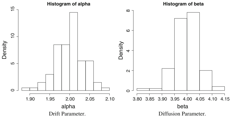
Fig. 1 Empirical Distribution of the estimators for \alpha and \beta .
