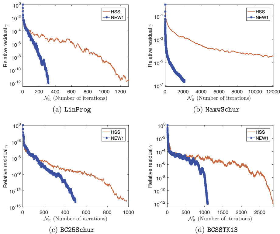
FIG. 5. Example 3. Convergence of PCG with the preconditioners NEW1 and HSS.
