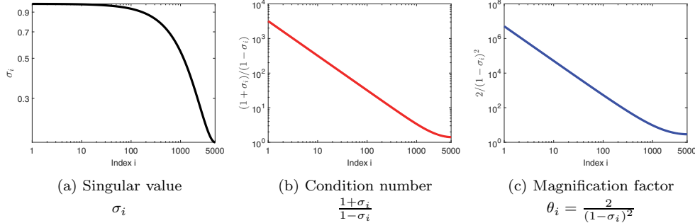
FIG. 1. For a 5-point discrete Laplacian matrix A evenly partitioned into a block 2 \times 2 form, (a) shows how the nonzero singular values \sigma_i of C decay, (b) shows how the condition number of the preconditioned matrix decays when the singular values smaller than or equal to \sigma_i are truncated, and (c) shows the factor that magnifies the decay.
