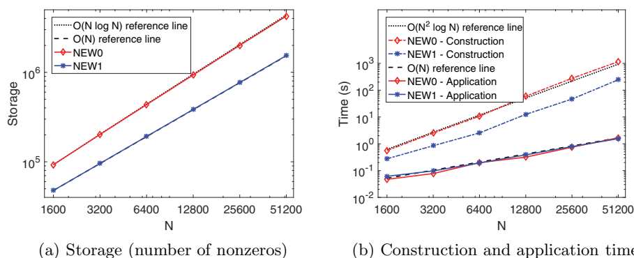
FIG. 3. Example 1. Storage for NEW0 and NEW1 and the runtime to construct them and to apply them to one vector.
