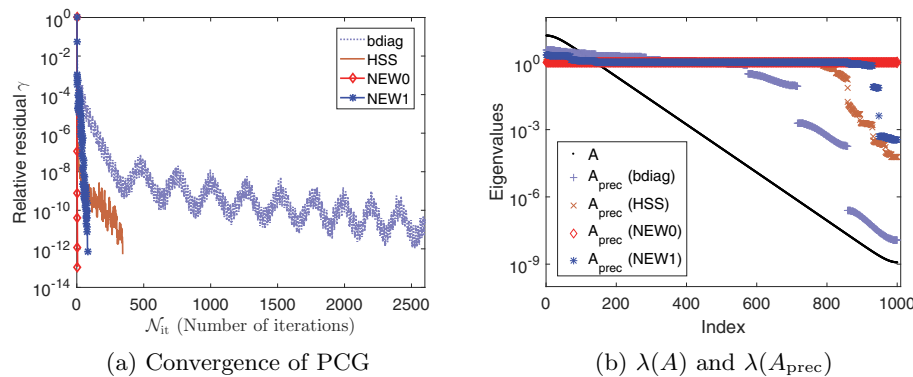
FIG. 4. Example 2. Convergence of PCG with the preconditioners for the matrix corresponding to \text{sech } \mu t , \mu = 0.2 in Table 3, and the eigenvalues before and after preconditioning.
