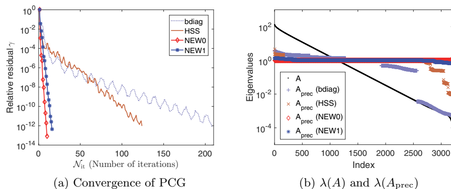
FIG. 2. Example 1. Convergence of PCG with the preconditioners for the matrix with N = 3200 , and the eigenvalues before and after preconditioning.
