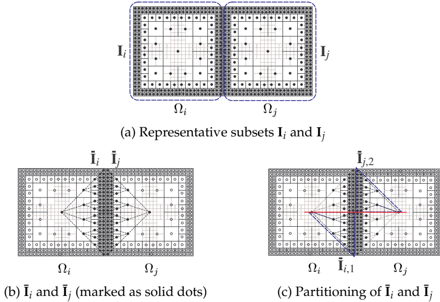
Figure 8: Study of the interactions between \bar{\mathbf{I}}_i and \bar{\mathbf{I}}_j for siblings i and j of \mathbf{T} .
