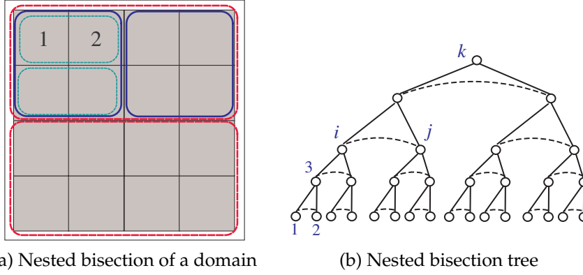
Figure 4: Nested bisection of a domain and the corresponding nested bisection tree T .
