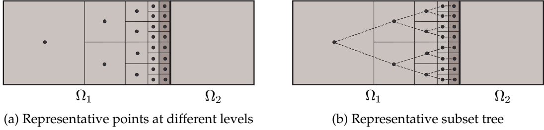
Figure 3: Representative points in \Omega_1 in the study of the interaction between \Omega_1 and \Omega_2 in the FMM and the corresponding representative subset tree for organizing the points. The locations of the representative points (marked as black dots) are for illustration purpose only.
