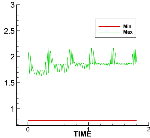
(d) With the entropy limiter (2.9). The time series of minimum and maximum values of \frac{p}{\rho^\gamma} = e^S in numerical solutions on 100 cells.
